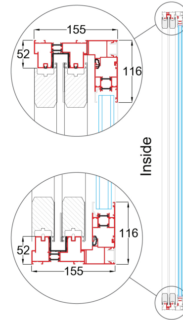
W6F Generic Section B-B
