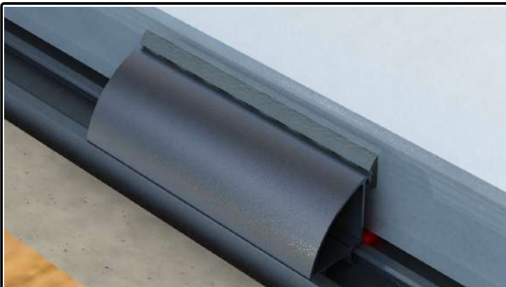
11) Install the bottomrail and handrail glazing bead bits and wedge gasket to hold the glass panel(s) temporarily.
