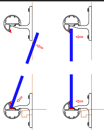
10) Seat a glass panel onto the packers and pivot the panel up to make contact with the fixed (E) gaskets.
