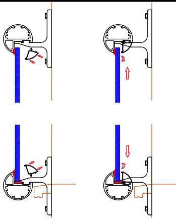
11) Install the bottomrail and handrail glazing bead bits and wedge gasket to hold the glass panel(s) temporarily.
