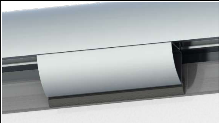
10) Seat a glass panel onto the packers and pivot the panel up to make contact with the fixed (E) gaskets.
